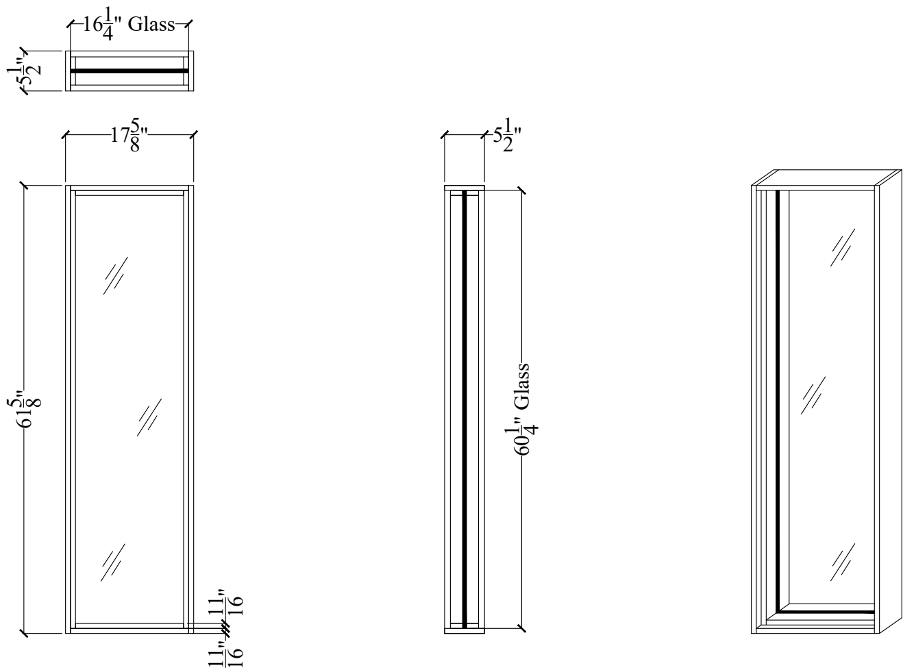
Window Assembly
